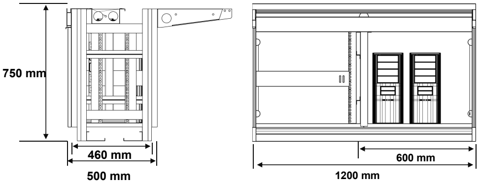
A set of bottom cabinet sizes
