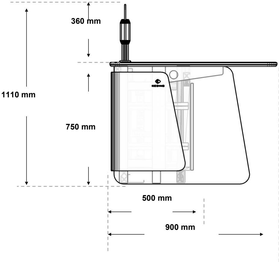
Side view
